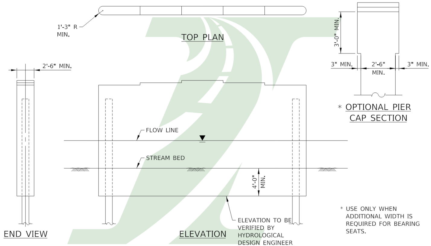
STREAM CROSSING EXPANSION PIER (ENCASED PILE TYPE)
