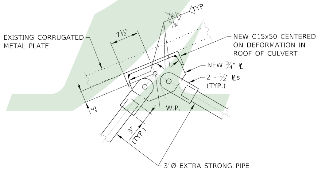
DETAIL 1
