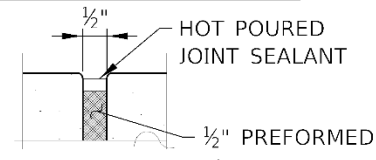
SEALING DETAIL
