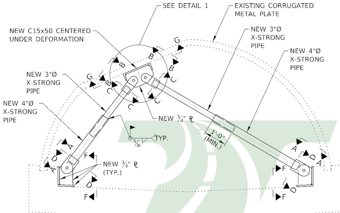
TYPICAL SECTION
