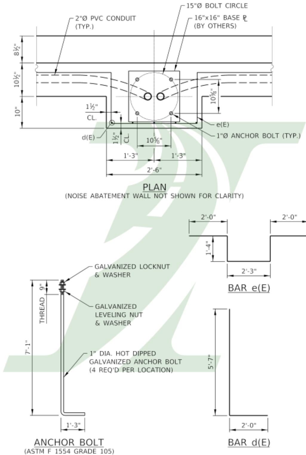
LIGHTPOLE DETAILS FOR 6FT BARRIER
