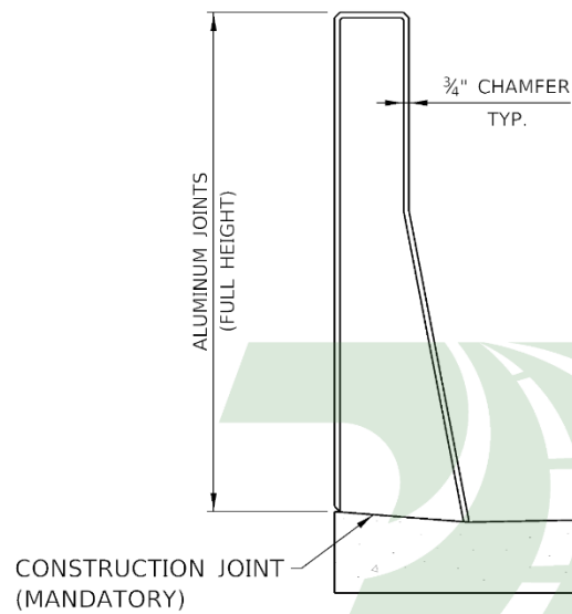
ALUMINUM JOINT DETAIL
