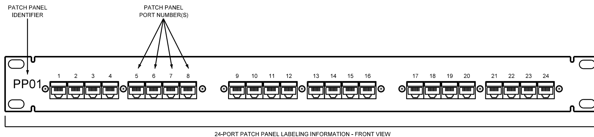
FIGURE B-18: COPPER PATCH PANEL LABELING SCHEME
