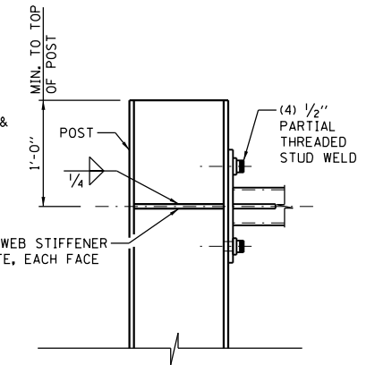
CONNECTION TO POST
