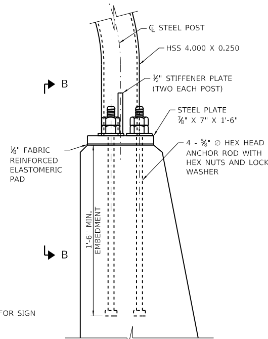
DETAIL B
