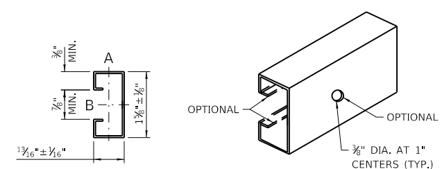
SUPPORTING CHANNEL DETAILS
