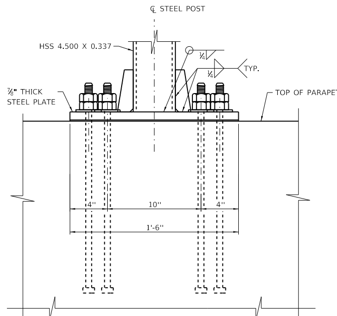
VIEW B-B
