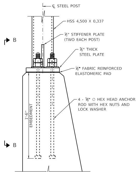
DETAIL A
