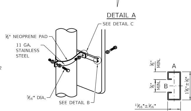
SIGN PANEL OVER 36" WIDE
